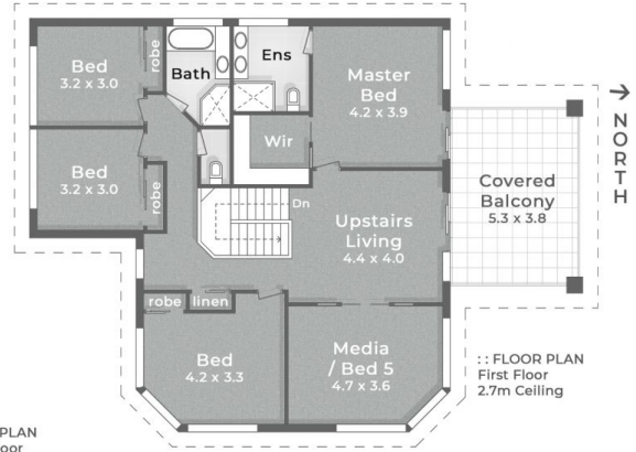
:: FLOOR PLAN Ground Floor 2.7m Ceiling
